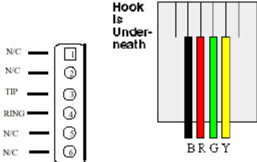
RJ11connector
